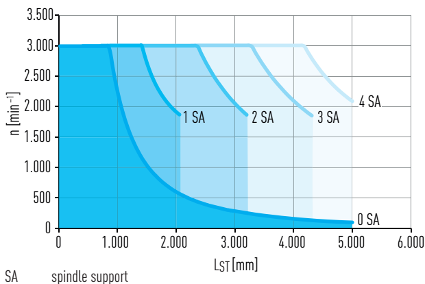
Fig. 8.5 Critical speed n over stroke length axis L_{\text{ST}}
