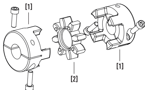
Fig. 18.32 Coupling components for linear modules HM-S and linear tables HT-S
