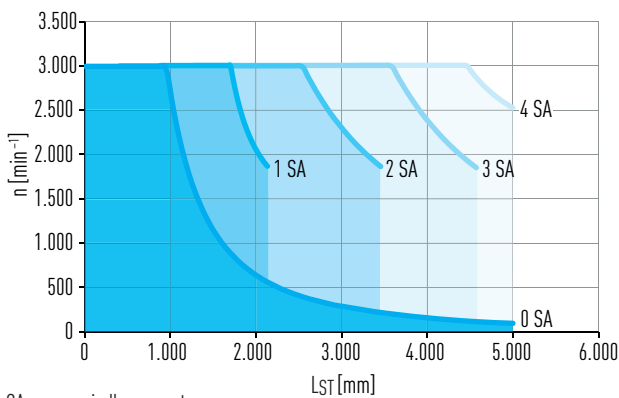
Fig. 8.8 Critical speed n over stroke length axis L_{\text{ST}}
