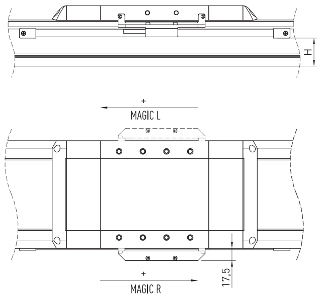
Fig. 17.2 Distance measuring system MAGIC – linear axes HT-B and HT-S
