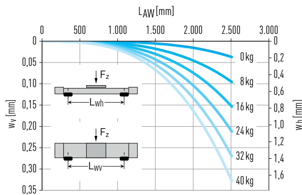
Fig. 8.2 Deflection w over unsupported axis length L_{\text{AW}} under payload F_z
