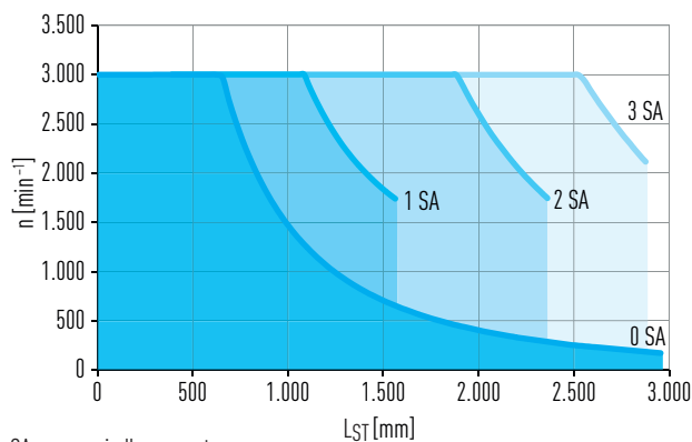
Fig. 6.3 Critical speed n over stroke length axis L_{\text{ST}}
