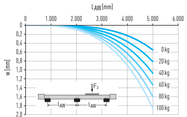
Fig. 5.8 Deflection w over unsupported axis length L_{AW} under payload F_z
