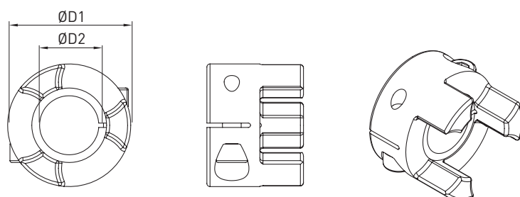
Fig. 18.33 Clamping hub
