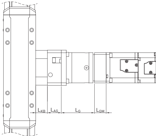
Fig. 18.10 HC cantilever axis motor connection with gears
