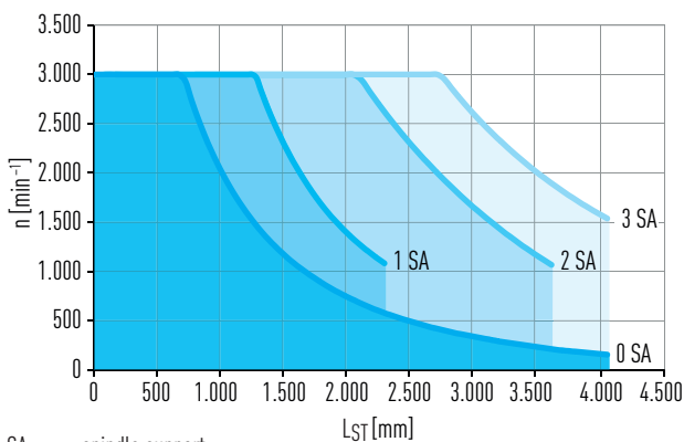
Fig. 6.5 Critical speed n over stroke length axis L_{\text{ST}}
