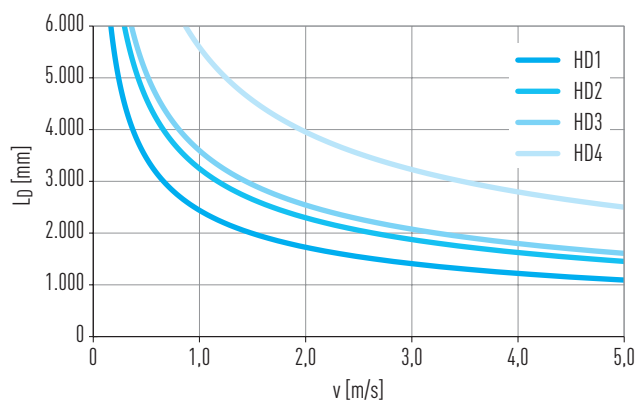
Fig. 11.1 Maximum distance between axes L_0 as a function of axis speed v
