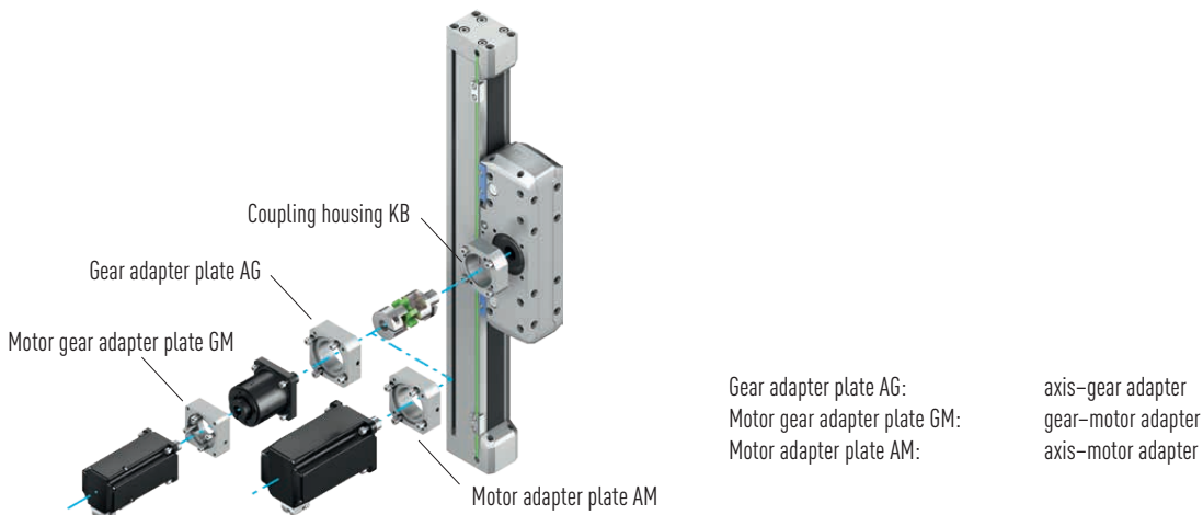
Fig. 18.4 Motor adapter for cantilever axes HC
