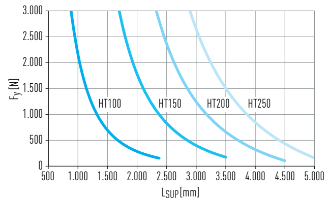
Fig. 3.17 HT: Maximum support spacing L_{sup} as a function of the force F_y
