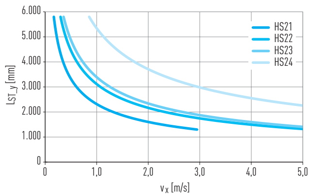
Fig. 12.1 Max X-axis speed v as a function of Y-axis stroke L_{ST}
