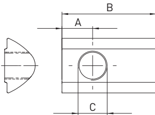
Fig. 19.4 Dimensional drawing of T nut
