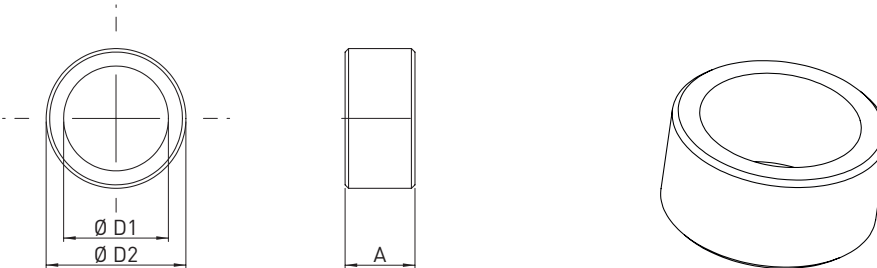
Fig. 19.5 Dimensional drawing of centring sleeve
