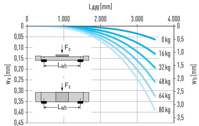
Fig. 8.4 Deflection w over unsupported axis length L_{\text{AW}} under payload F_z
