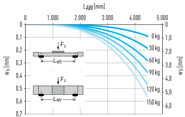
Fig. 8.6 Deflection w over unsupported axis length L_{\text{AW}} under payload F_z
