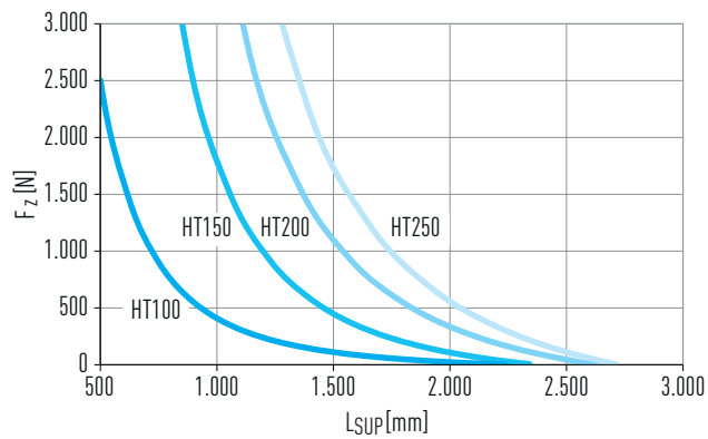
Fig. 3.16 HT: Maximum support spacing L_{sup} as a function of the force F_z
