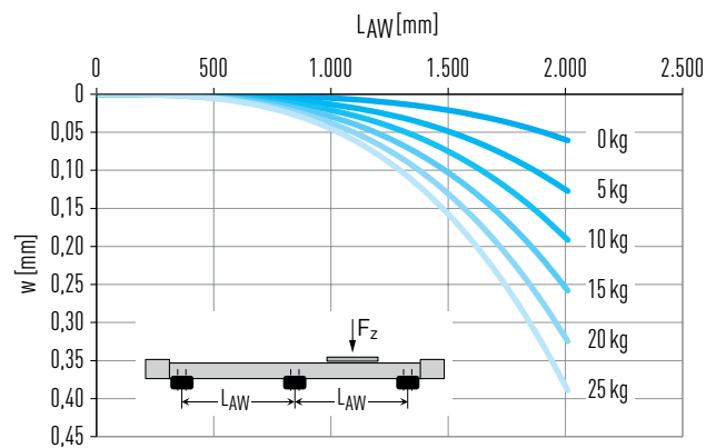
Fig. 6.4 Deflection w over unsupported axis length L_{\text{AW}} under payload F_z
