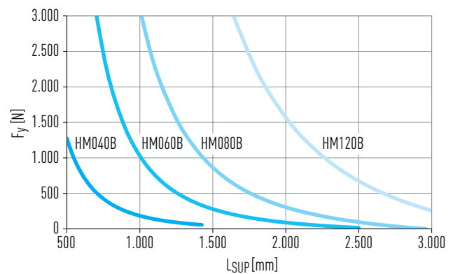
Fig. 3.13 HM-B: Maximum support spacing L_{SUP} as a function of the force F_y
