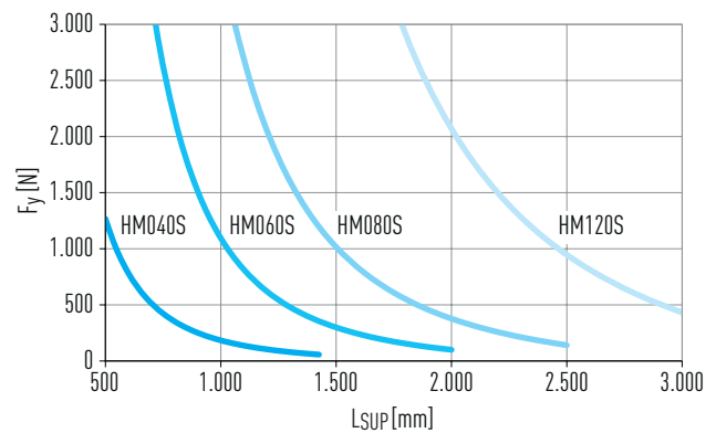
Fig. 3.15 HM-S: Maximum support spacing L_{SUP} as a function of the force F_y
