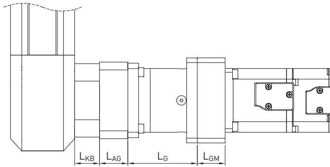
Fig. 18.8 HM-B linear module motor connection with gears
