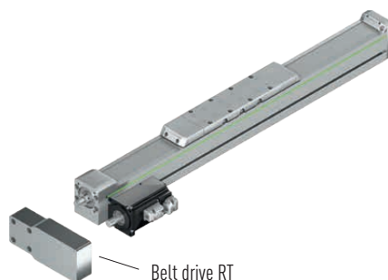
Fig. 18.22 Motor adapter for linear modules HM-S with belt drive
