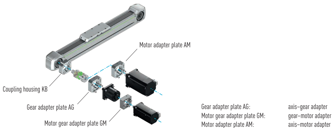
Fig. 18.1 Motor adapter for linear modules HM-B
