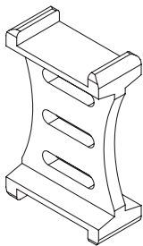
Fig. 19.14 Separator for energy chain
