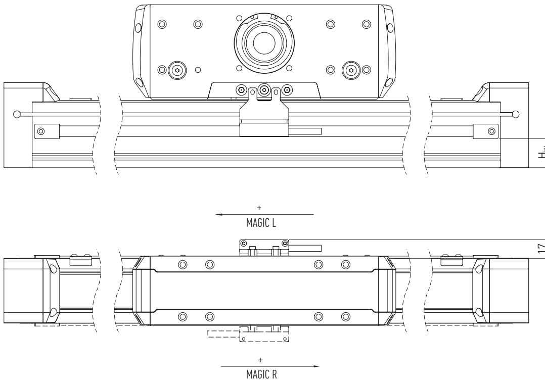
Fig. 17.3 Distance measuring system MAGIC – cantilever axis HC
