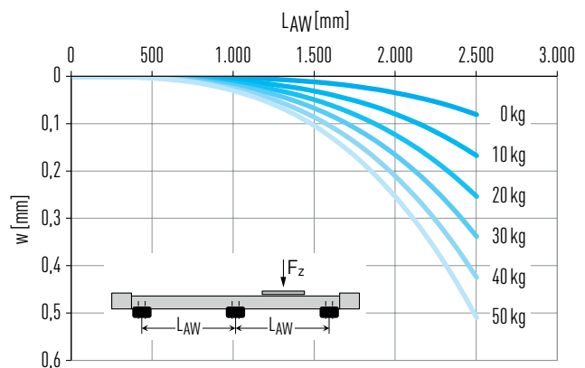
Fig. 6.6 Deflection w over unsupported axis length L_{\text{AW}} under payload F_z
