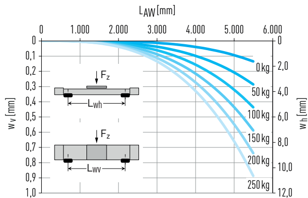
Fig. 8.7 Deflection w over unsupported axis length L_{\text{Aw}} under payload F_z
