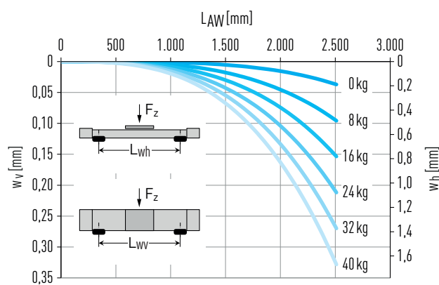
Fig. 7.2 Deflection w over unsupported axis length L_{AW} under payload F_z
