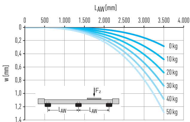
Fig. 5.6 Deflection w over unsupported axis length L_{AW} under payload F_z
