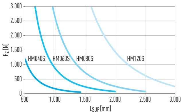
Fig. 3.14 HM-S: Maximum support spacing L_{SUP} as a function of the force F_z
