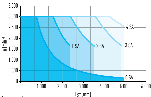
Fig. 6.7 Critical speed n over stroke length axis L_{ST}
