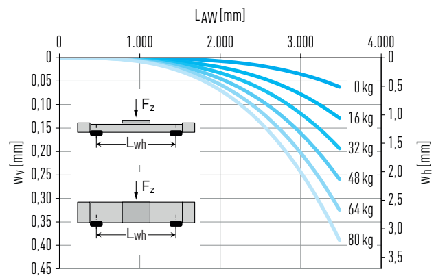
Fig. 7.4 Deflection w over unsupported axis length L_{AW} under payload F_z
