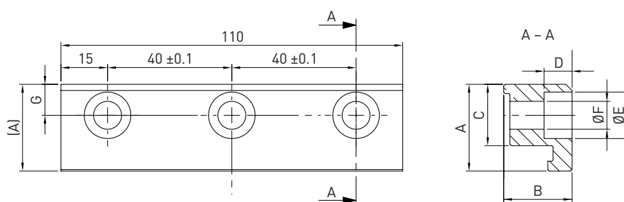
Fig. 19.3 Dimensional drawing of long clamping profile
