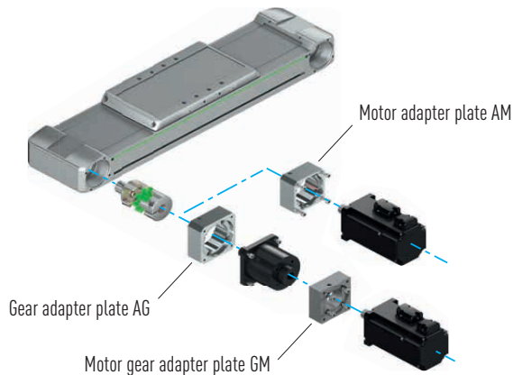
Fig. 18.3 Motor adapter for linear tables HT-B
