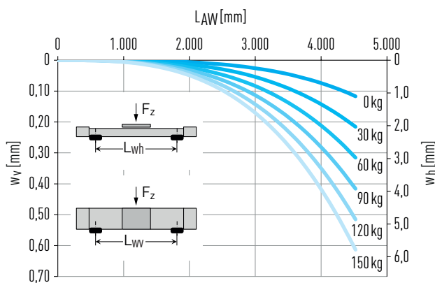
Fig. 9.4 Deflection w over unsupported axis length L_{\text{AW}} under payload F_z
