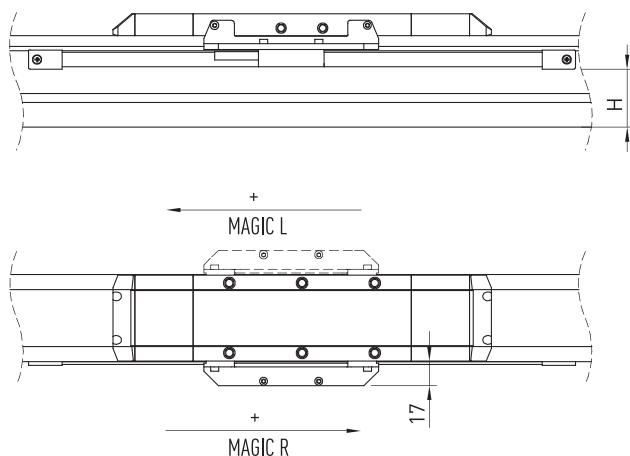
Fig. 17.1 Distance measuring system MAGIC – linear axes HM-B and HM-S
