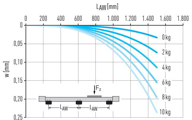
Fig. 5.2 Deflection w over unsupported axis length L_{AW} under payload F_z
