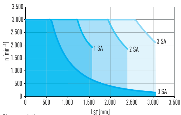
Fig. 8.1 Critical speed n over stroke length axis L_{\text{ST}}
