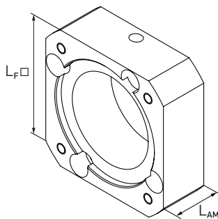
Fig. 18.12 Motor adapter plate AM for linear modules HM-B, linear tables HT-B and cantilever axes HC without gears
