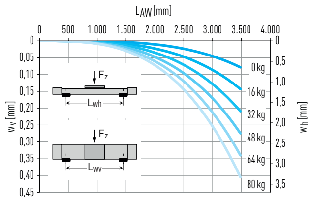
Fig. 9.2 Deflection w over unsupported axis length L_{\text{AW}} under payload F_z
