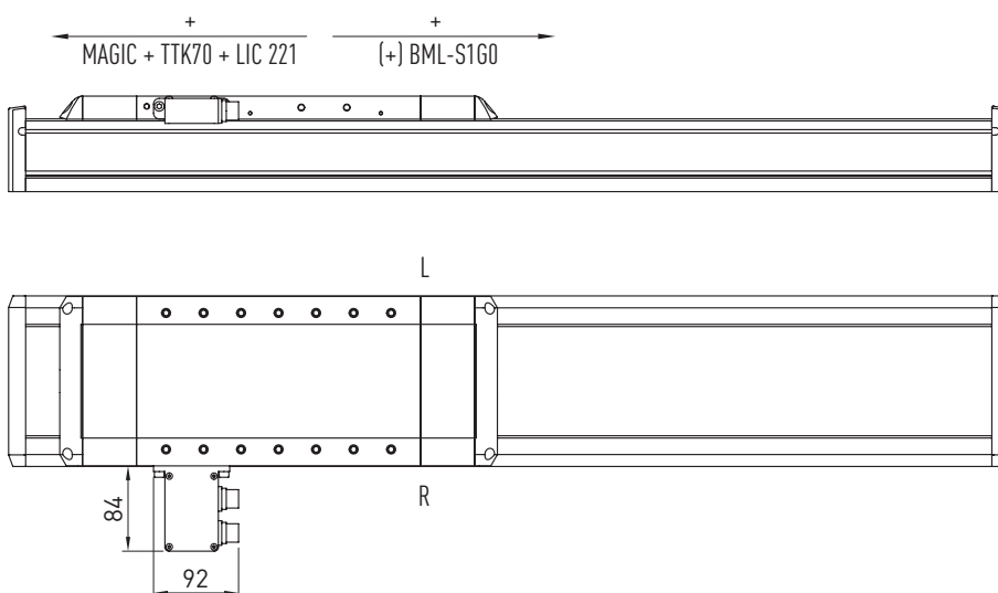
Fig. 17.4 Linear axis HT-L: connection interface "D" – connector right/rear
