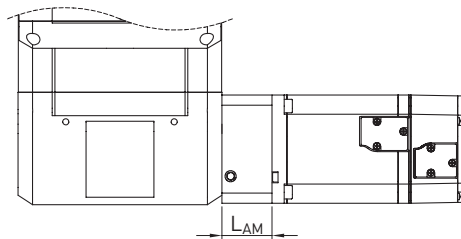
Fig. 18.6 HT-B linear table motor connection without gears
