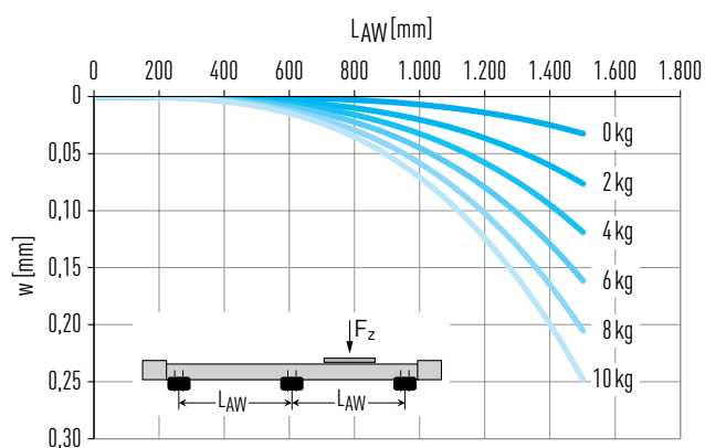
Fig. 6.2 Deflection w over unsupported axis length L_{AW} under payload F_z
