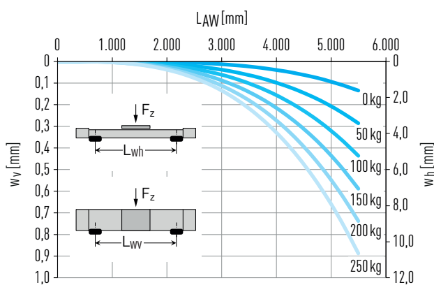
Fig. 7.8 Deflection w over unsupported axis length L_{AW} under payload F_z
