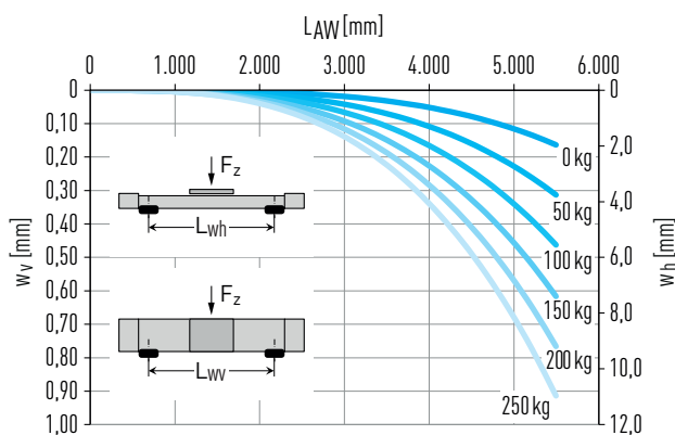
Fig. 9.6 Deflection w over unsupported axis length L_{\text{AW}} under payload F_z
