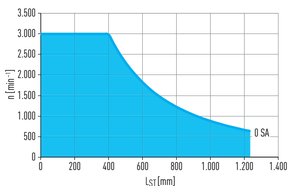
Fig. 6.1 Critical speed n over stroke length axis L_{ST}
