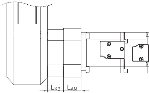
Fig. 18.5 HM-B linear module motor connection without gears
