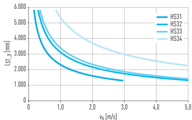
Fig. 13.1 Max X-axis speed v as a function of Y-axis stroke L_{ST}
