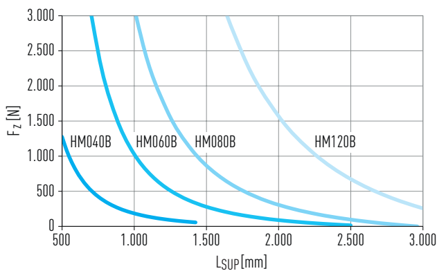
Fig. 3.12 HM-B: Maximum support spacing L_{SUP} as a function of the force F_z
