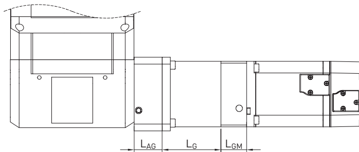
Fig. 18.9 HT-B linear table motor connection with gears
