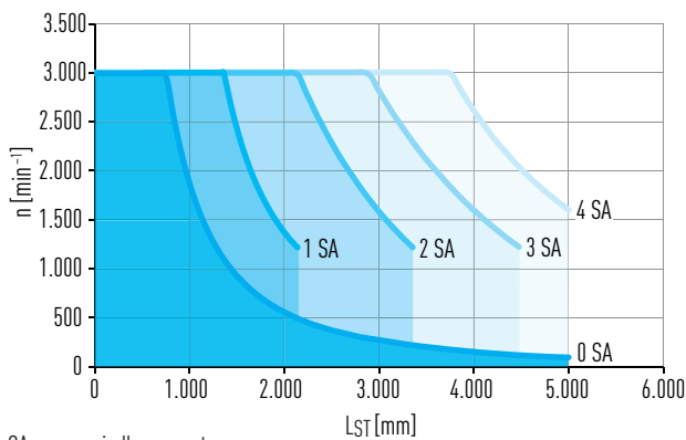
Fig. 8.3 Critical speed n over stroke length axis L_{\text{ST}}
