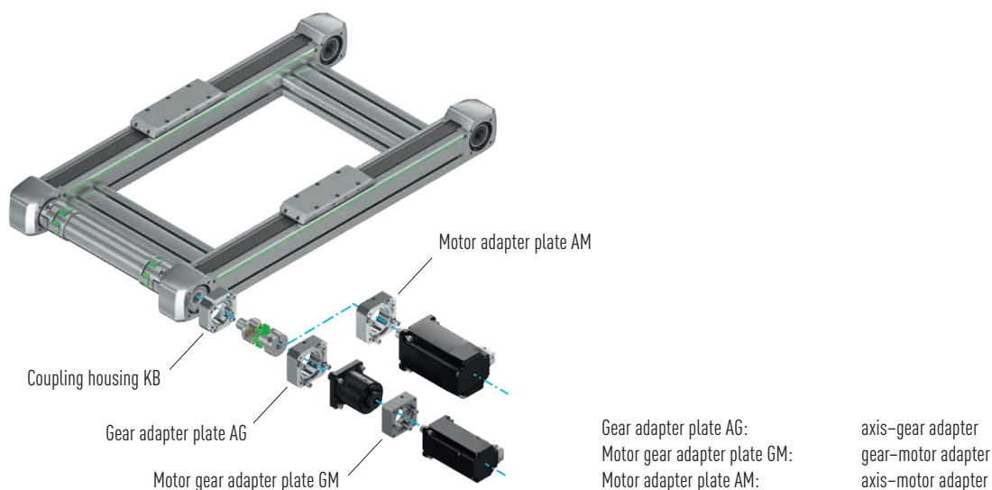
Fig. 18.2 Motor adapter for double axes HD
