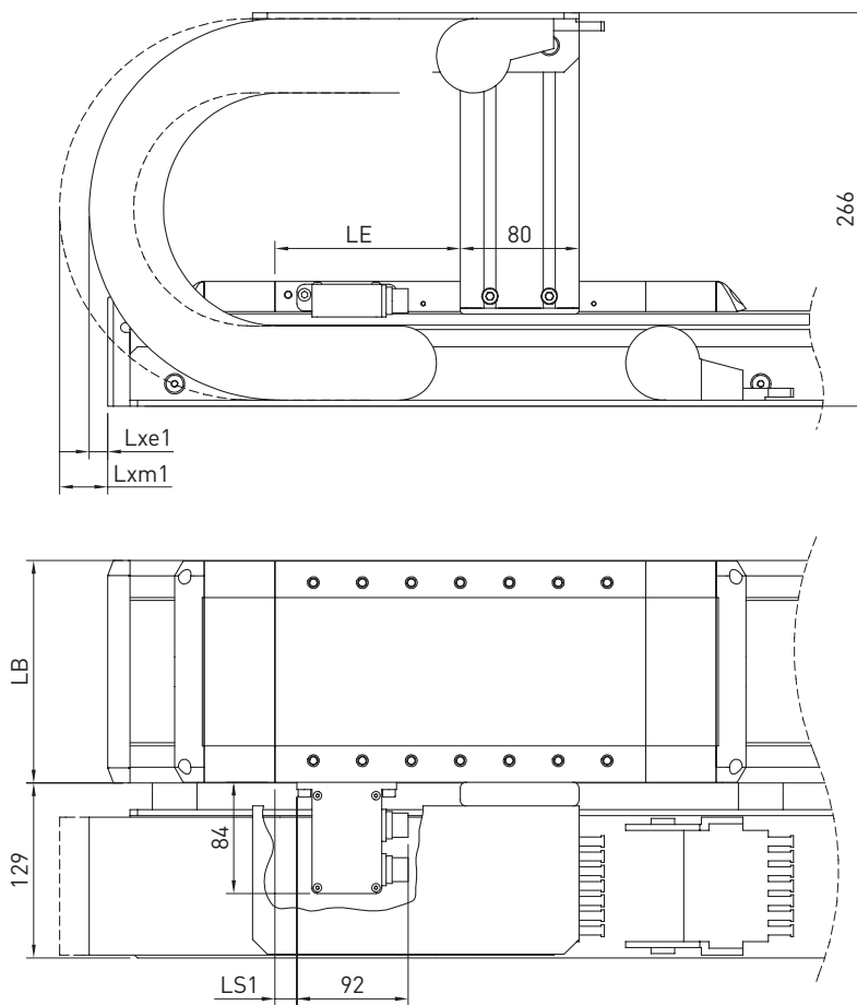
Fig. 18.38 Linear motor axes HT-L: “D” and “F” options – connector right/front, mirrored also applies to “C” and “E” options – connector left/front
