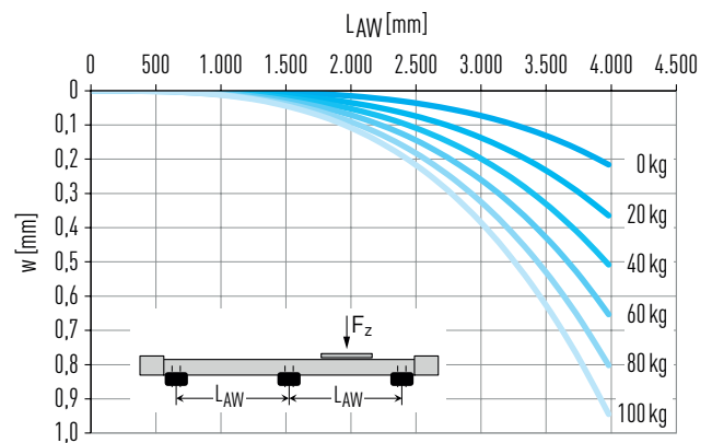
Fig. 6.8 Deflection w over unsupported axis length L_{AW} under payload F_z
