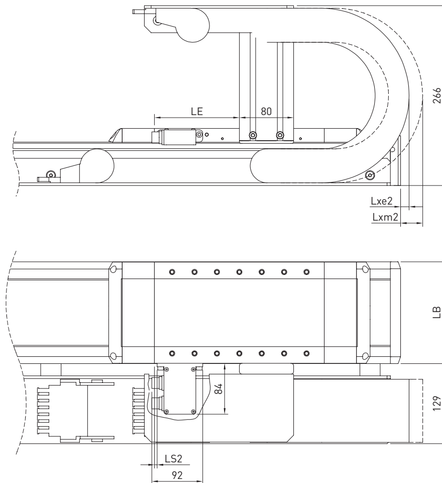
Fig. 18.39 Linear motor axes HT-L: “R” and “B” options – connector right/front, mirrored also applies to “L” and “A” options – connector left/front
