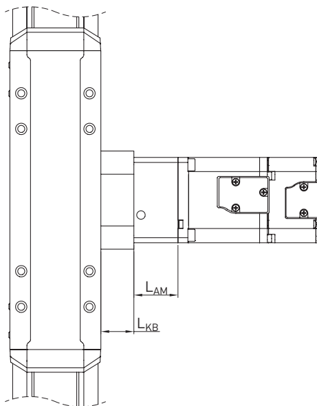
Fig. 18.7 HC cantilever axis motor connection without gears
