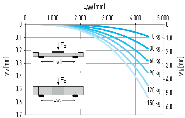
Fig. 7.6 Deflection w over unsupported axis length L_{AW} under payload F_z
