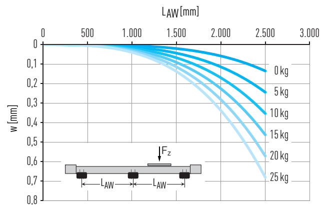
Fig. 5.4 Deflection w over unsupported axis length L_{AW} under payload F_z
